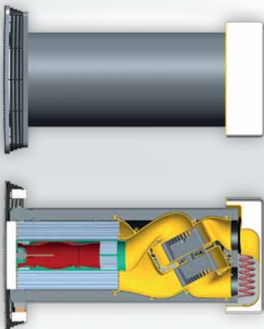
Sectional view Air 70
